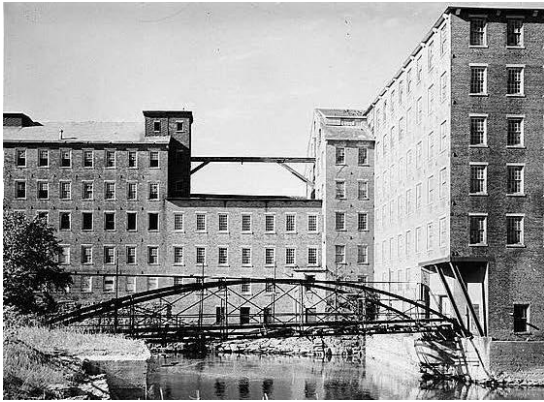
Figure 70: Moseley Bowstring Bridge - One of the few extant examples of this type of bridge; crossed over the Sugar River between Mill #6 and the former Monadnock Mill power plant and carried pipes and workers (Library of Congress)
